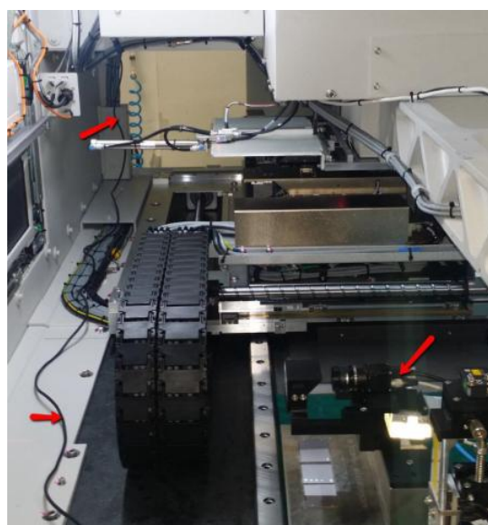
Figure 9 Camera Cable Routing (Reference Only)
