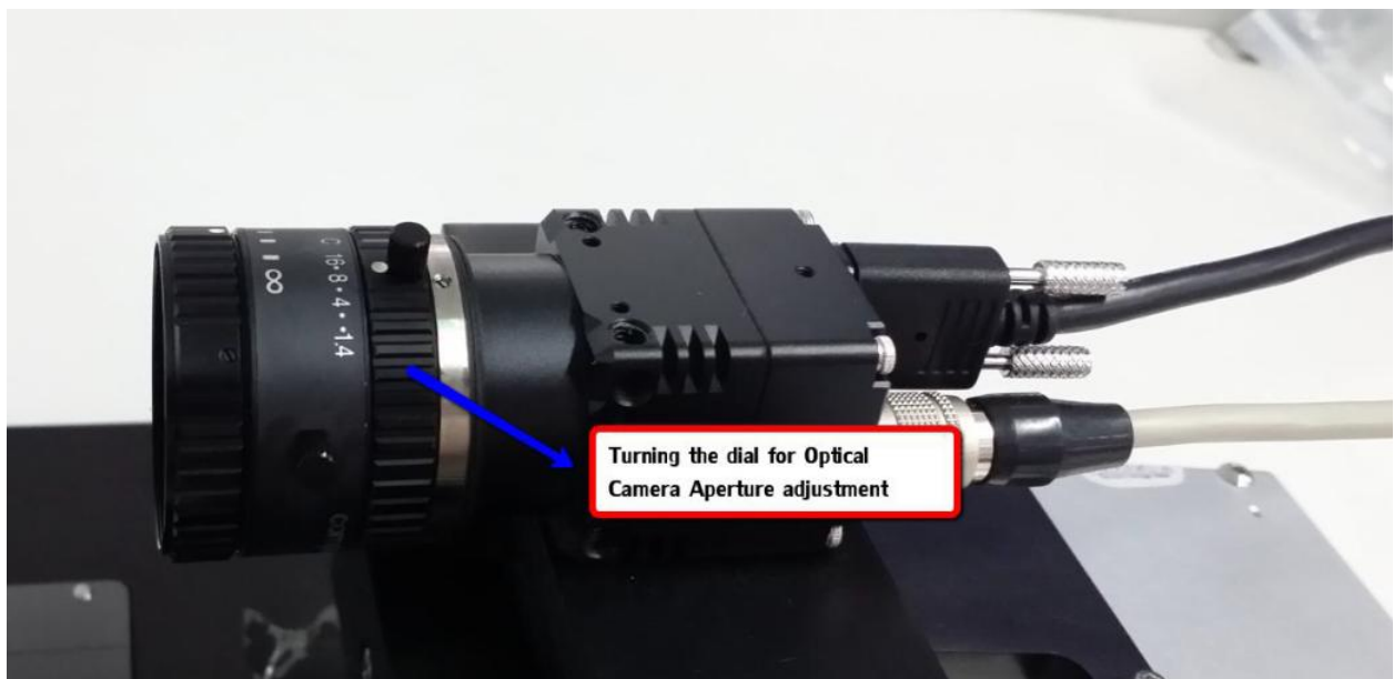
Figure 58 Aperture Dial Turning
